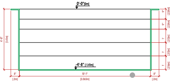
CORTE TRANSVERSAL |CROSS SECTION|LA COUPE TRANSVERSALE
