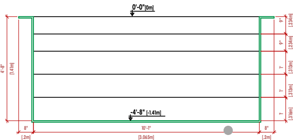
CORTE TRANSVERSAL |CROSS SECTION|LA COUPE TRANSVERSALE
