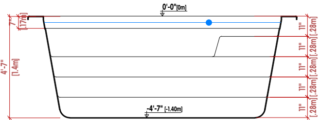
● CORTE TRANSVERSAL | CROSS SECTION | LA COUPE TRANSVERSALE
