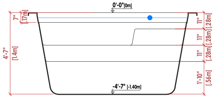
● CORTE TRANSVERSAL |CROSS SECTION|LA COUPE TRANSVERSALE
