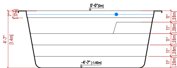
● CORTE TRANSVERSAL | CROSS SECTION | LA COUPE TRANSVERSALE
