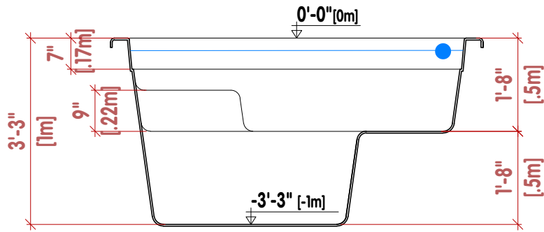
● CORTE TRANSVERSAL | CROSS SECTION | LA COUPE TRANSVERSALE
